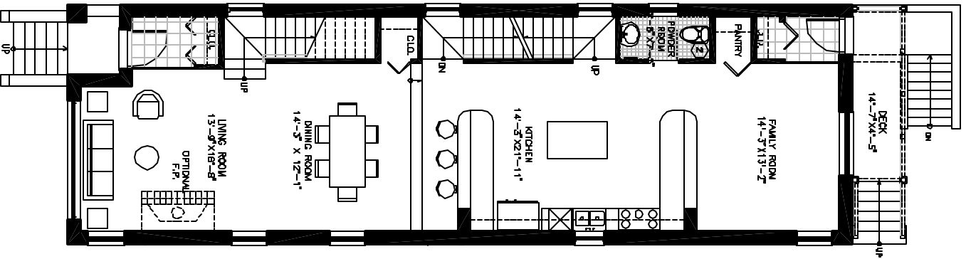
FIRST FLOOR PLAN OPTION 3 AREA = 1,285 SQ.FT.
